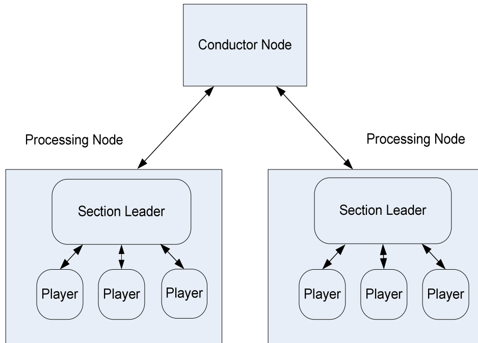
Figure 1: Orchestrate Architecture
